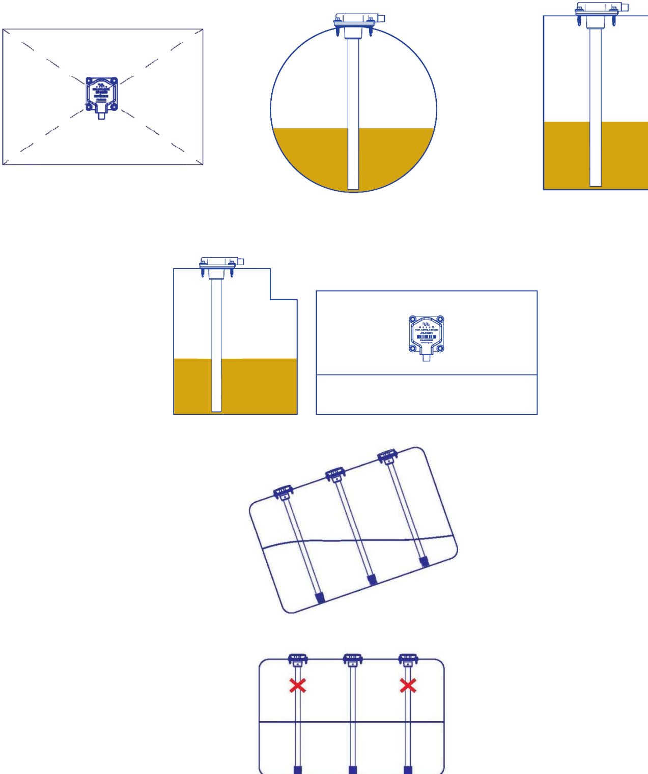
Figure 1. Selecting the location to install sensor
