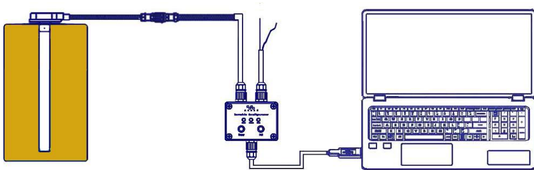
Figure 6 . The USB of the portable configuration device is connected to the computer, and power is supplied to the fuel level sensor through the computer, which is convenient for calibration.
