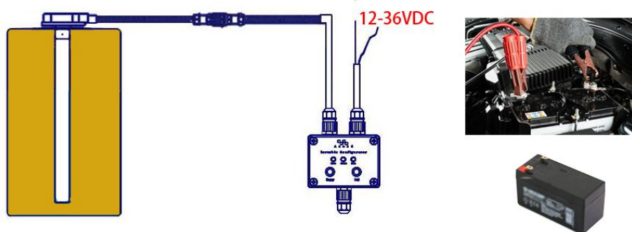
Figure 7 . Portable configurator power cable connected to truck battery or battery
