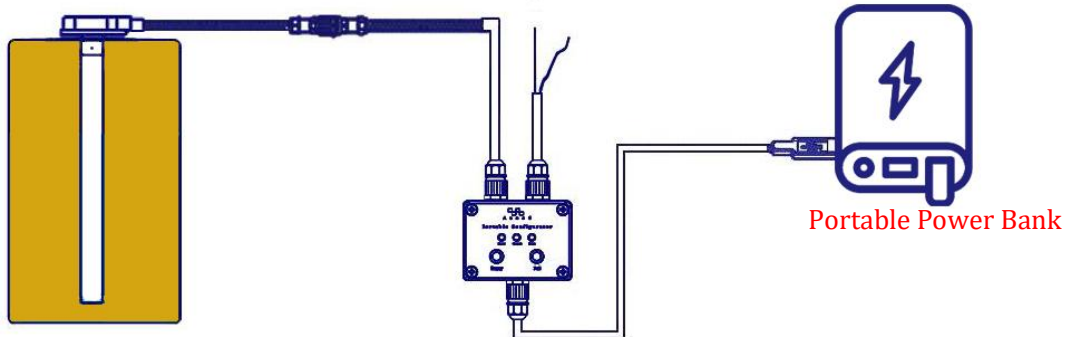
Figure 5. Connect the portable configurator USB to the power bank, and use the power bank to power the fuel level sensor.
