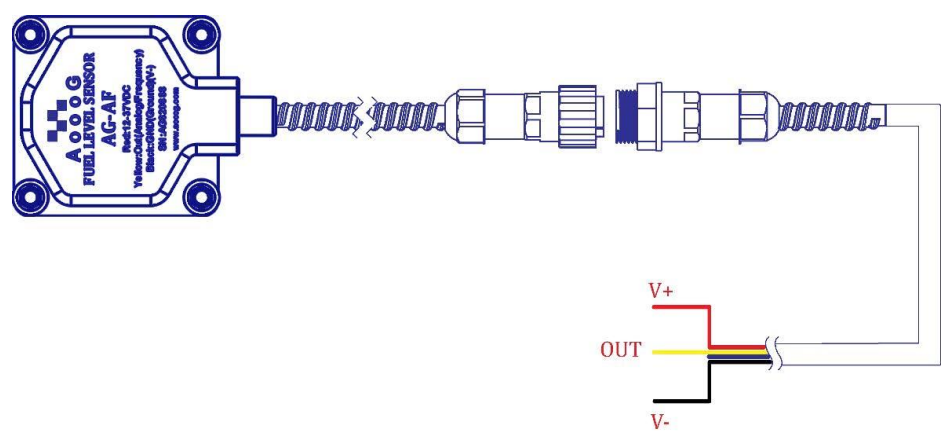
Figure 12. Wiring diagram of Analog and Frequency output signals
