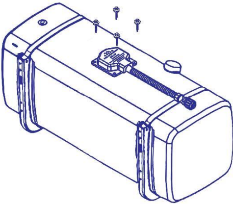
Figure 10 . Put sensor into the tank
