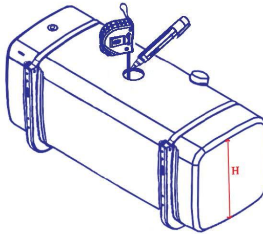
Figure 3. Measuring the tank depth
