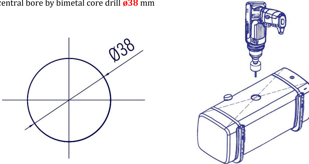
Figure 2. Drilling the selected hole
