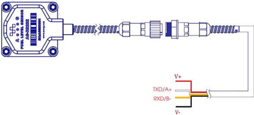
Figure 11. Wiring diagram of RS485 and RS232 output signals
