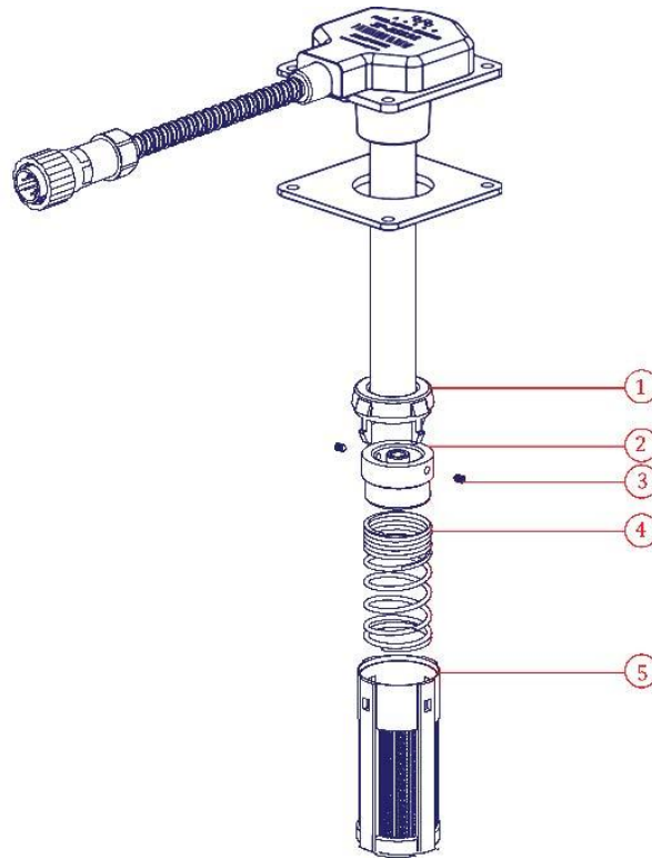
Figure 8 . Procedure for Installing the Screen Filter
